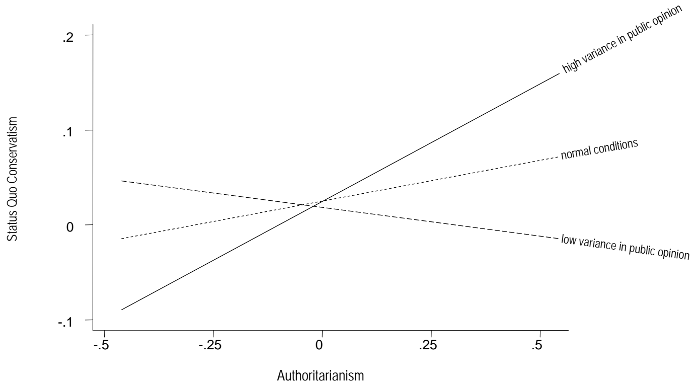
Figure E.1: Effects of Authoritarianism on Status Quo Conservatism Given Varying Experience of Normative Threat
